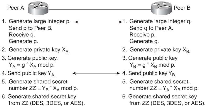
Figure 1-9 DH Key Exchange
