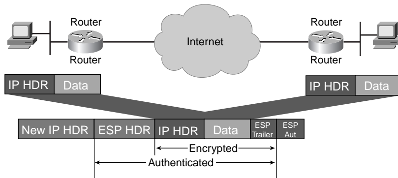
Figure 1-18 ESP Protocol
