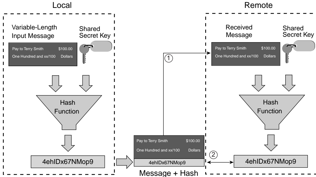
Figure 1-11 HMAC
