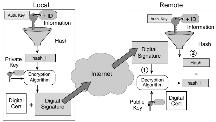
Figure 1-14 RSA Signatures
